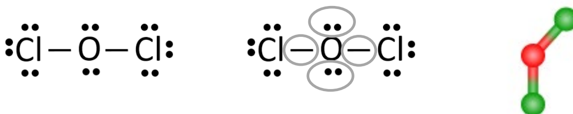
Figure 2: A) The Lewis structure for \text{OCl}_2 drawn where it appears to be linear. B) The Lewis structure for \text{OCl}_2 with electron groups circled. C) The molecular model for \text{OCl}_2 shows bent molecular geometry.
