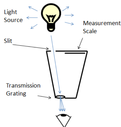
Figure 1: Spectroscope
