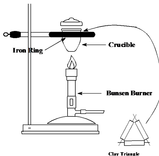
Figure 2: Crucible Heating
