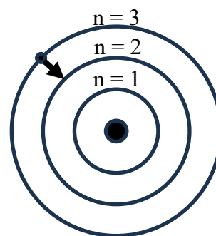
Figure 2: Bohr Model
